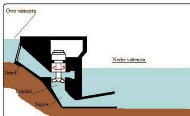
Kaplan-turbin (propellerturbin) < 75 m
